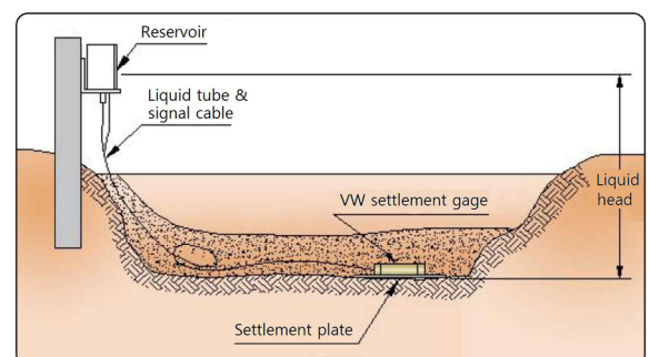
[Installation of VW settlement gage]
